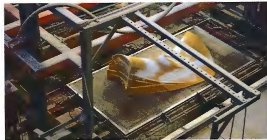
Polyurethane foam mold on the heat forming table
